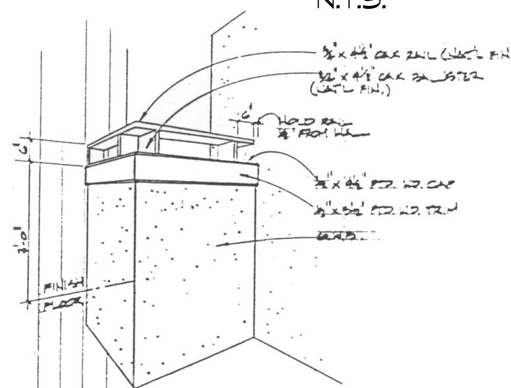
Interior Balcony Rail Detail #8 / D4 N.T.S.
